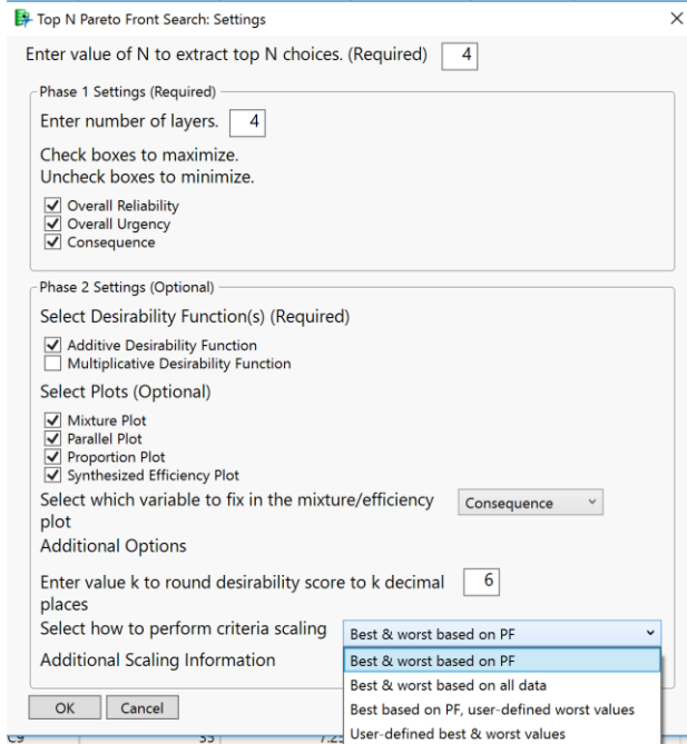
Figure 6. TopN-PFS Settings window: Scaling Options
