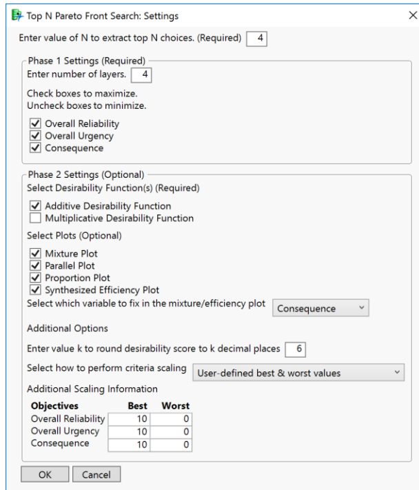
Figure 8. TopN-PFS settings window filled in for stockpile prioritization example
