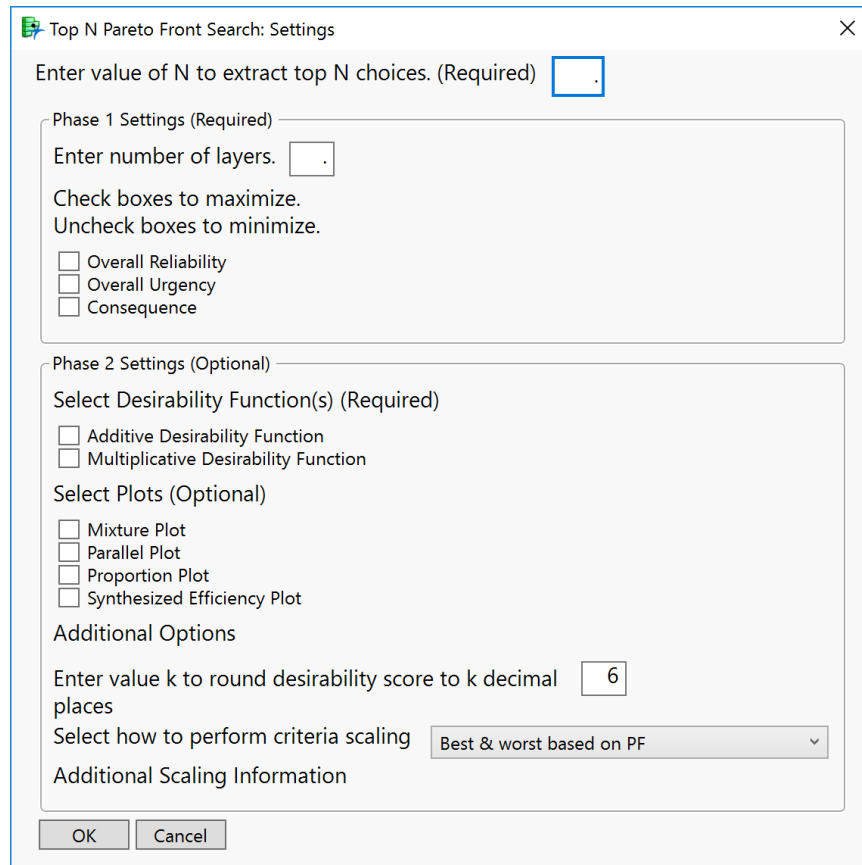
Figure 5. TopN-PFS Settings Window
