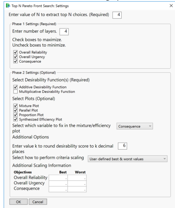
Figure 7. TopN-PFS Settings Window: Scaling Option 4 selected
