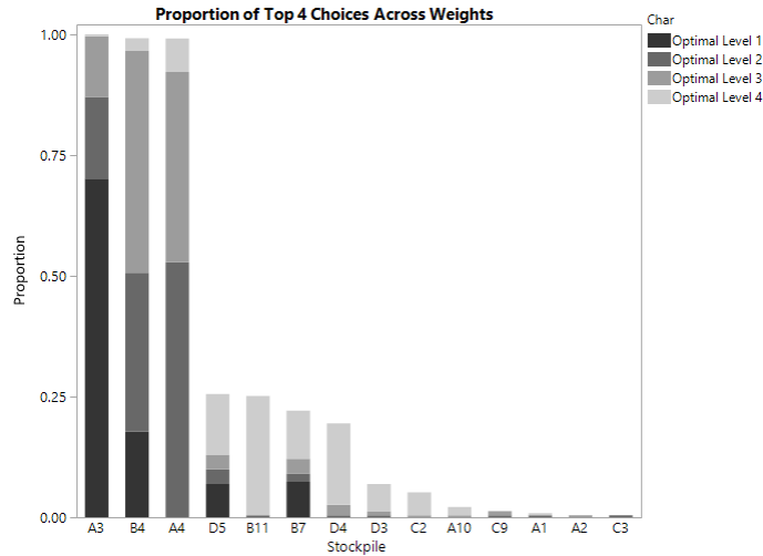
Figure 12. Proportion plot for stockpile prioritization example
