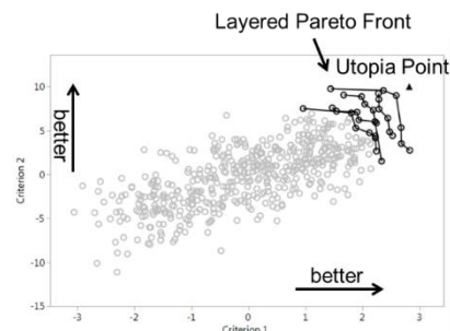
Figure 1. Layered PF with 5 layers where both criteria are optimized by maximization
