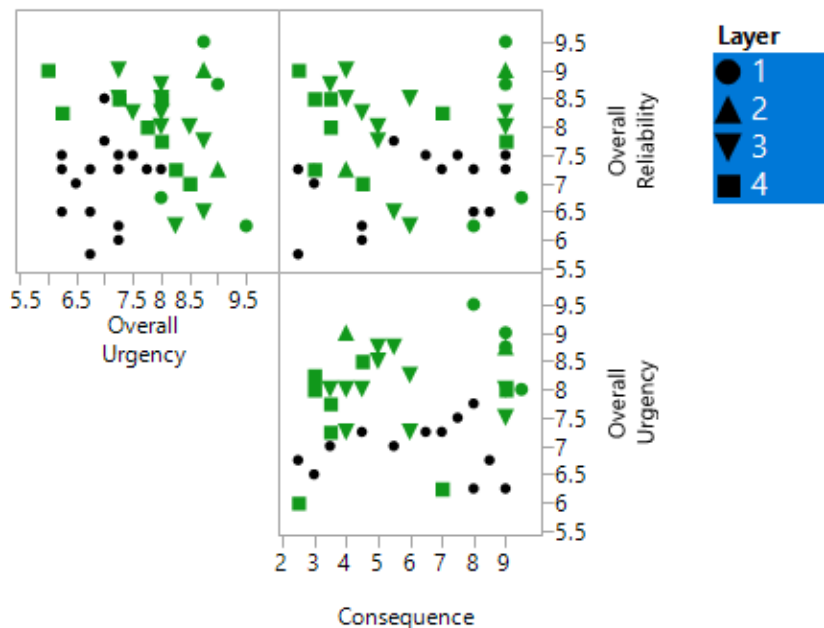
Figure 10. Top 4 Pareto front layers for the stockpile prioritization example
